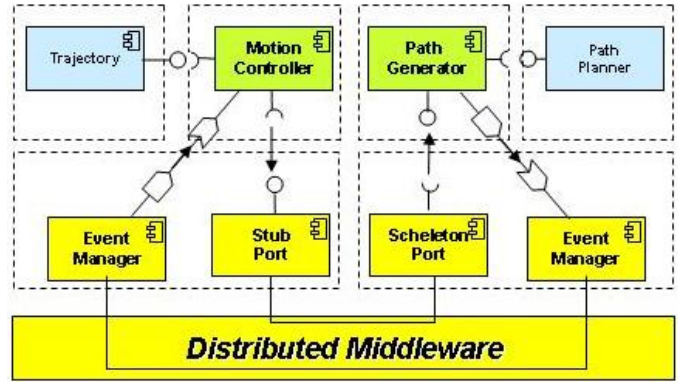
Fig. 4. Container services for distributed component interactions
