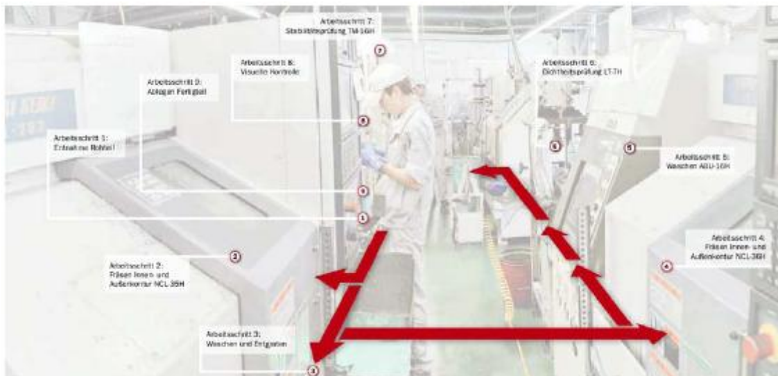
Figure 1: Chaku-chaku line as established at Robert Bosch GmbH
